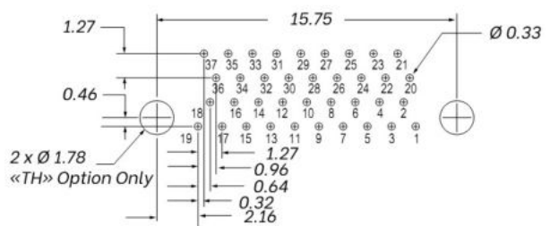
37 Contacts
