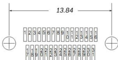
31 Contacts
