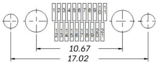
21 Contacts
