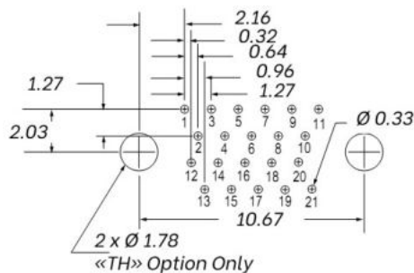
21 Contacts
