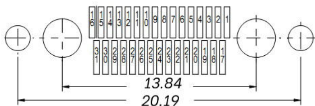
31 Contacts
