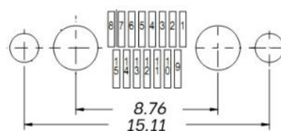
15 Contacts
