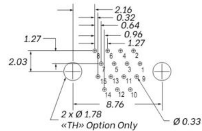
15 Contacts
