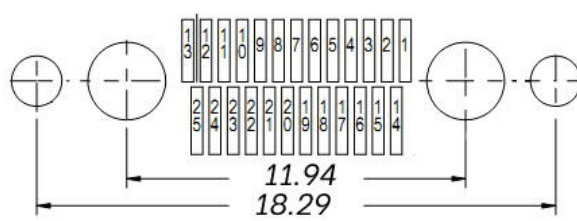
25 Contacts
