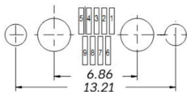
9 Contacts
