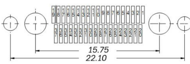
37 Contacts
