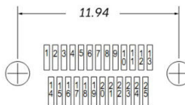
25 Contacts
