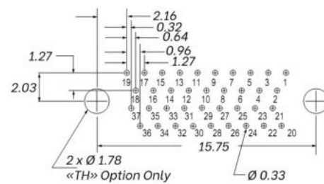
37 Contacts
