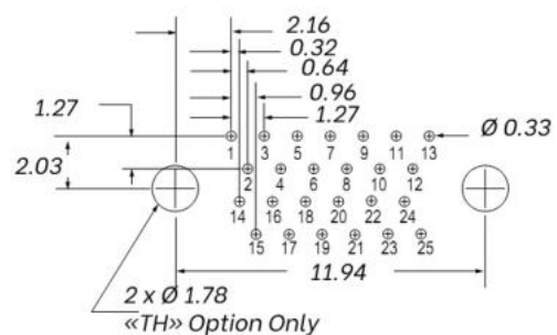
25 Contacts
