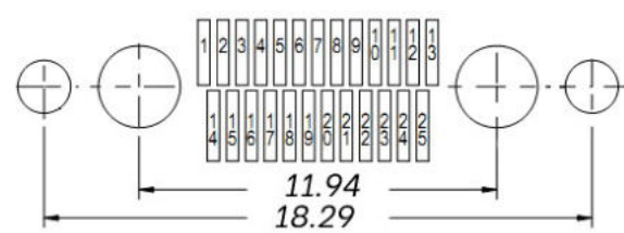
25 Contacts
