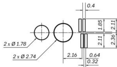
Pad Dimensions
