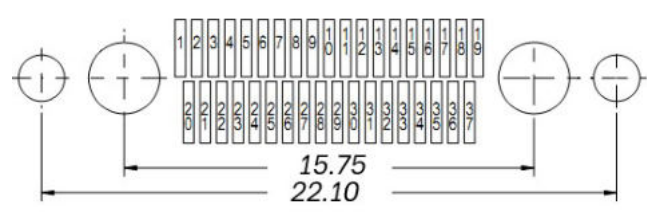
37 Contacts
