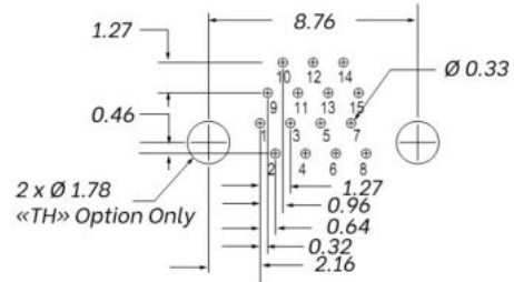
15 Contacts
