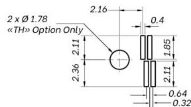
Pad Dimensions
